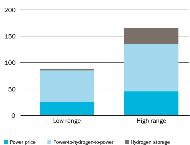
Figure 9. Illustration of cost developments for solar PV combined with batteries in sunny areas and up to four hours' storage (USD/MWh) (left). Costs (high and low) for renewable hydrogen converted back to power via fuel cell plant in 2030 (EUR/MWh) (right). Low Emissions Scenario 2019.
