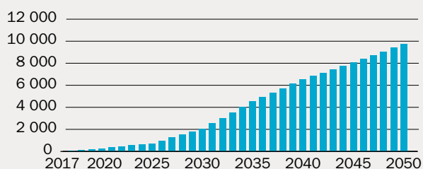
Figure 25. Battery capacity is expected to increase significantly towards 2050, driven by the automotive industry (left). Smart charging of electric cars smoothens the daily profile of the power systems – example from 2040 (right). Statkraft analysis.
