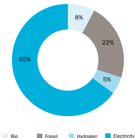
Figure 21. End-use energy in buildings in 2050 by source for the Low Emissions Scenario and 1.5-degree pathway for Europe. Statkraft analyses.
