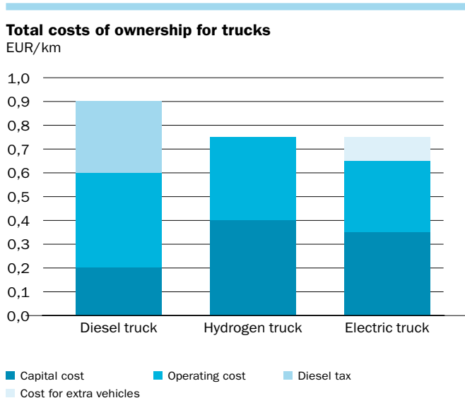
Figure 19. Lifetime cost for heavier trucks in 2030, assuming driving pattern suitable for hydrogen and electricity respectively 38 . Statkraft analyses.
