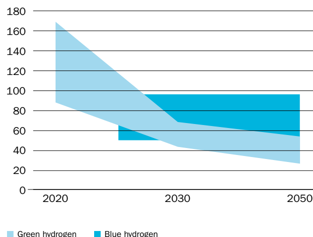
Figure 17. Illustration of cost developments for electrolyzers, external sources (left). Total cost of producing green and blue hydrogen (right). Statkraft analyses and IHS Cera 2018. 36
