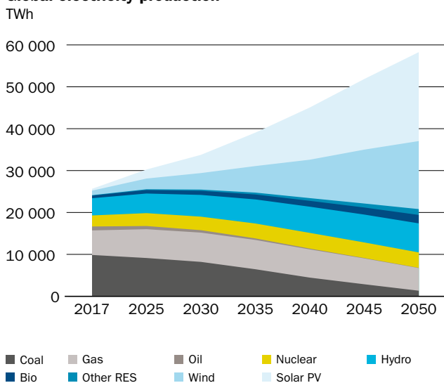
Figure 5. Electricity production to 2050 in TWh (left). The electricity share of final energy use per sector today and in 2050 and compound average annual growth rate per sector (right).
