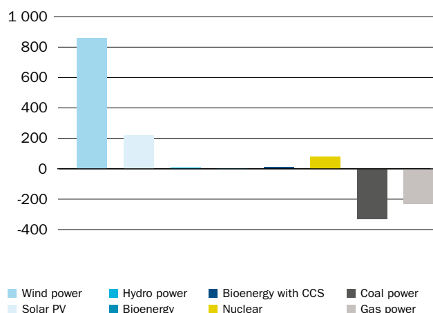
Figure 24. Changes in power generation in Europe in a 1.5-degree pathway compared to the Low Emissions Scenario in 2050 (TWh). Statkraft analysis.
