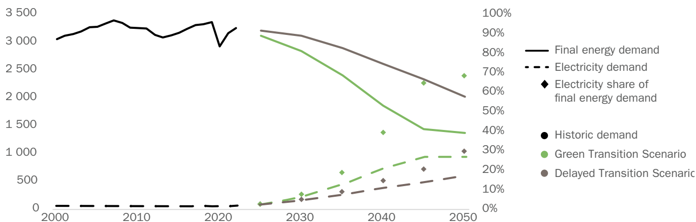
42 Final energy and electricity demand in Transport historic and to 2050 for Green and Delayed scenarios (line, TWh) and share of electricity in total final energy (dots, %).
