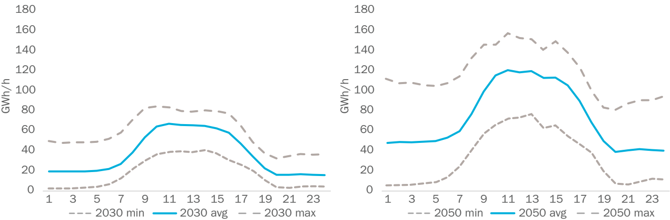
45 German solar and wind power generation during 24 hours in 2030 (left) and 2050 (right) (TWh).
